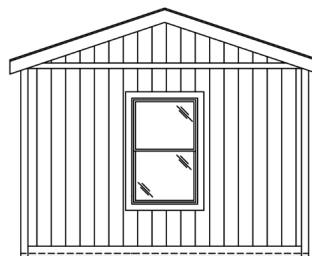
FRONT ENDWALL
